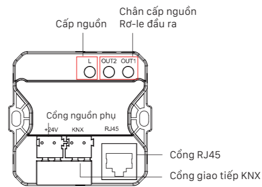
Source-KNX Power Interface
