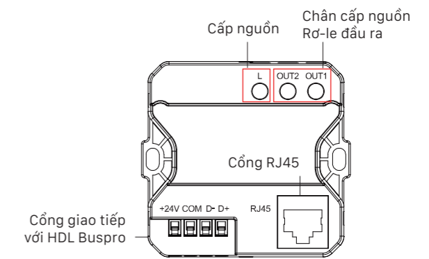
Source-Buspro Power Interface
